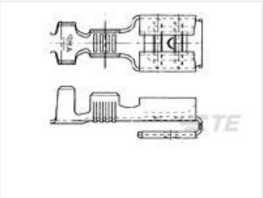
TE 产品编号160739-2 250 FASTON,PIGGYBACK REC.,18-14 AWG,TPBR
