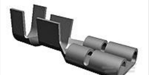
TE 产品编号63306-1 250 FASTON REC 18-14 AWG BR
