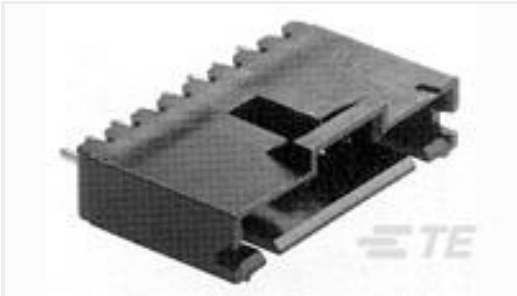
TE 产品编号5-104362-1 02 MTE HDR SRST LATCH W/HLDWN AU038
