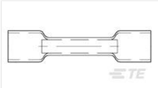
TE 产品编号603502-3 PRE-INSUL SEALED SPLICE 22-16
