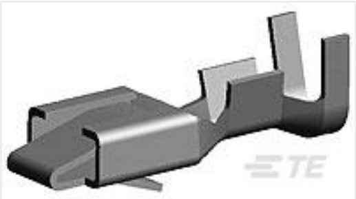
TE 产品编号640417-2 BLADE REC 250 18-14AWG TPBR
