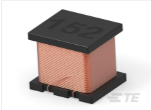
TE 产品编号2176641-1 3627C 575047 R12 20%
