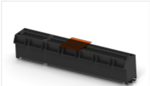
TE 产品编号4-2337939-3 PCIE GEN4 CON,SMT,98POS,15u", MYLAR,HT
