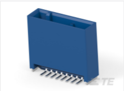
TE 产品编号2311396-3 8POS,TAB0.5X0.4,HDR ASSY,180DEG, COD C
