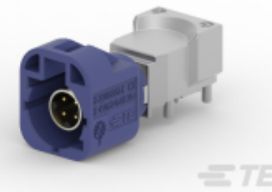
TE 产品编号2286546-3 HSD,HDR ASSY,90DEG,COD C
