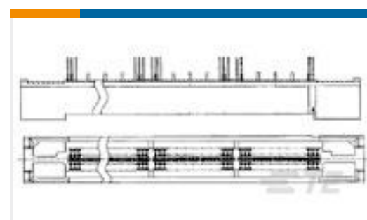
TE 产品编号767143-3 MICT,R/A,RCPT,114,ASY,062,30AU
