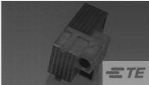
TE 产品编号5120641-1 12 ROW HM RA REC ASY 072P RGHT
