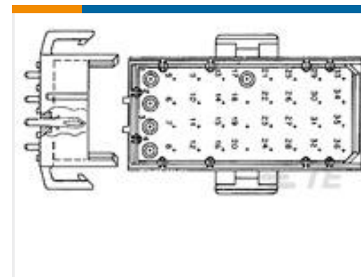
TE 产品编号640499-4 04P MR HDR ASSY V0
