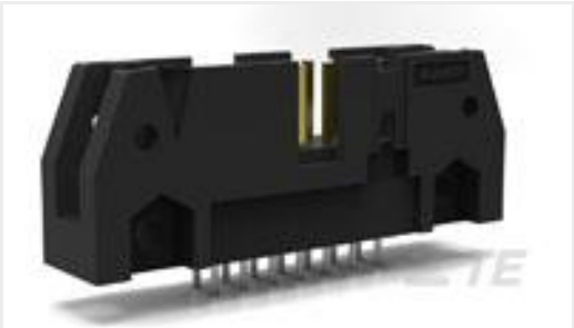
TE 产品编号5102153-6 A/L UNIV HDR 26P VERT
