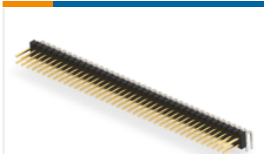
TE 产品编号 9-146309-0 80 MODII HDR DRRA B/A .100CL
