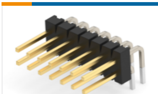
TE 产品编号 5-146309-7 14 MODII HDR DRRA B/A .100CL
