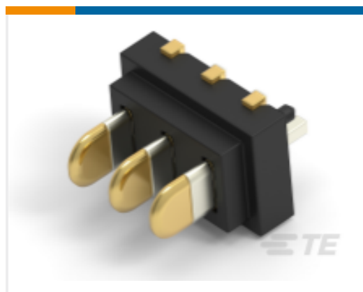
TE 产品编号2315312-1 BATTERY BLOCK CONN. PLUG ASSY
