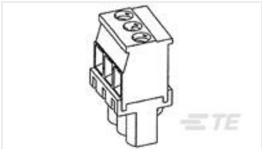
TE 产品编号1-1986374-0 Str Plug, 3.81mm, Green, RH, 1
