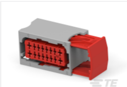
TE 产品编号185760-6 16W HYBRID RCPT HSG GRAY
