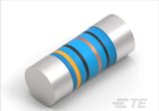
TE 产品编号2176315-4 MELF SMA_A 180R 0.1% 15PPM 0204 0.4W
