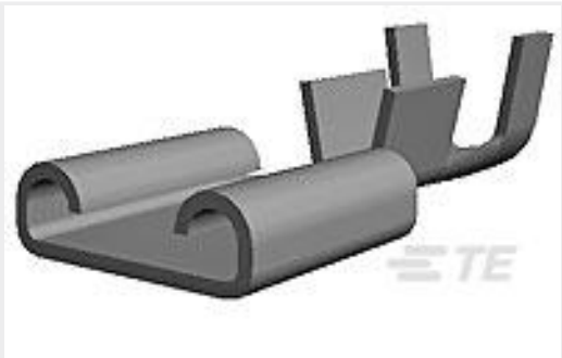
TE 产品编号5-160506-8 250 FASTON REC 20-16 AWG TPBZ
