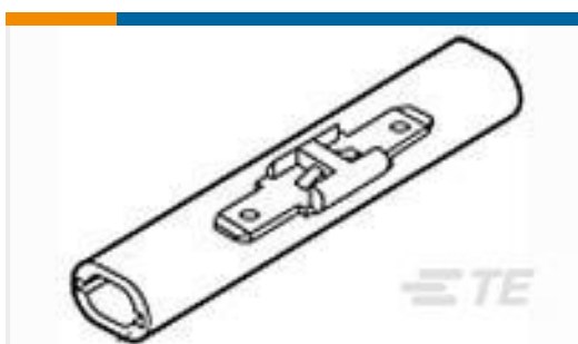
TE 产品编号360035-1 .187 INLINE SPLICE ASSY
