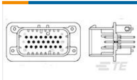
TE 产品编号776231-1 35POS, PIN DIA 1.3, HDR ASSY, 180DEG, COD 1
