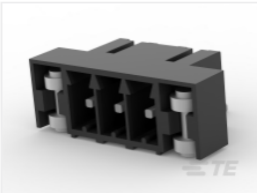
TE 产品编号2213933-3 SMT TB R/A HEADER, RET, 3.5MM, 3 POS
