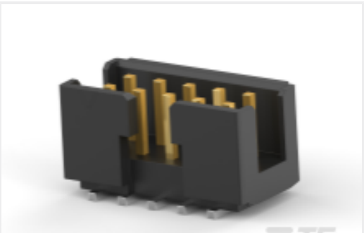
TE 产品编号1-2373376-0 10P,2MM,SHRD HDR,DRV, SMD,0.1 AU,TB
