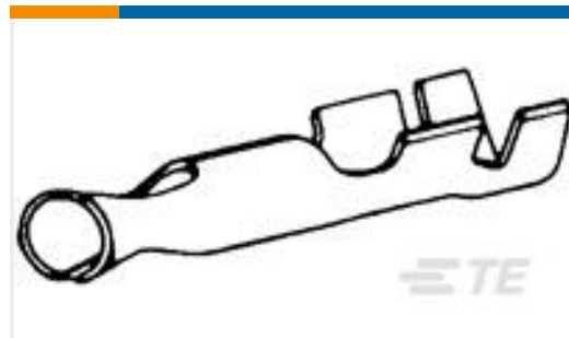
TE 产品编号42428-5 PIN TERMINAL RECEPTACLE 24-20 AWG TPPHBZ
