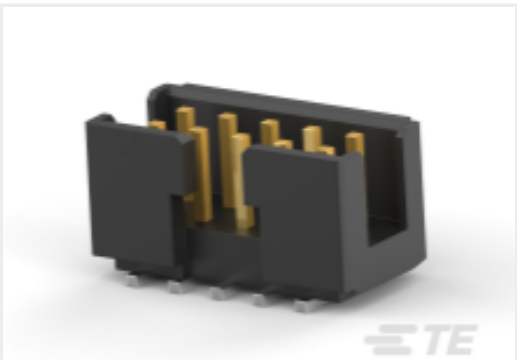
TE 产品编号1-2373376-0 10P, 2MM, SHRD HDR, DRVT, SMD, 0.1 AU, TB
