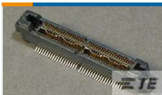
TE 产品编号5767056-2 MICT,260,PLUG,76,ASSY,PDNI
