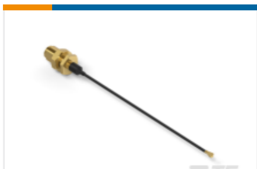
TE 产品编号2016694-2 RF CA,UMCC4 TO SMA JACK,1.13MM, L100MM
