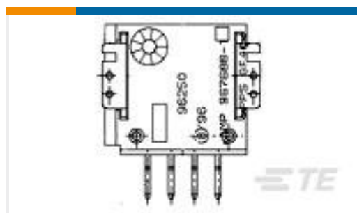
TE 产品编号967688-1 4pos MQS .63 header 90deg SMD
