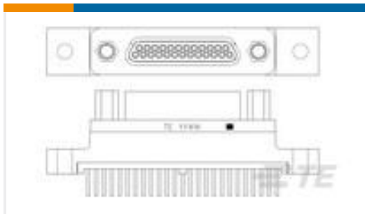
TE 产品编号1532269-4 M83513/22-D01NP = MCKS-N1-P-25PST1
