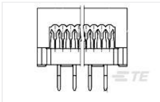
TE 产品编号5746613-2 14 DIP PLUG CONN-W/COVER
