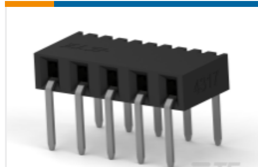
TE 产品编号2307706-5 5P,2MM,B-B,REC,SRHZ,2.1,0.38AU,TR
