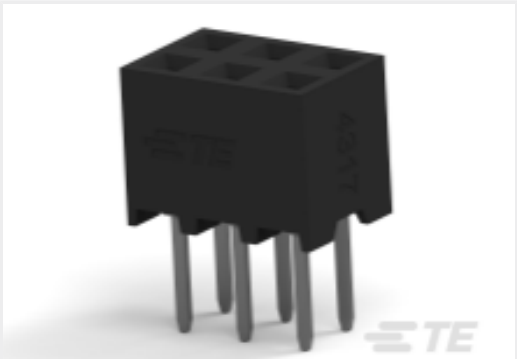
TE 产品编号2314822-6 6P,2MM,B-B,REC,DRVT,2.7,0.76AU,TB
