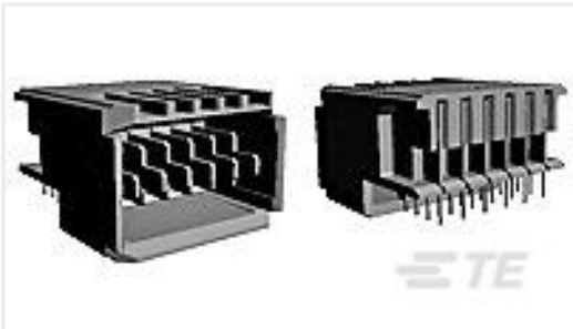
TE 产品编号5646956-1 UPM EXPANDED PIN ASSEMBLY
