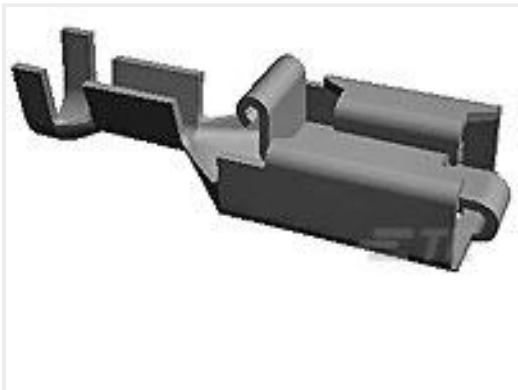
TE 产品编号154717-1 PL 250 REC TERMINAL 13-11 AWG BR
