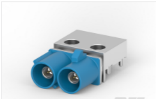
TE 产品编号5-2287923-3 FAKRA, 2 POS, EXT-EDGE, ASS'Y 12 O'CLOCK
