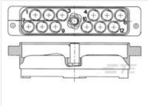
TE 产品编号1604798-2 ASY,RCPT,PWB MT,12 POS
