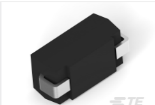
TE 产品编号2176323-7 SMV 2W 330K 5%
