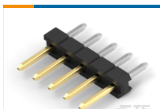
TE 产品编号2355177-6 6P,2MM,BRK HDR,SRVT,2.8,0.38AU,TB
