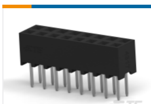
TE 产品编号1-2314813-6 16P,2MM,B-B,REC,DRVT,2.0,0.38AU, TB,W/CAP
