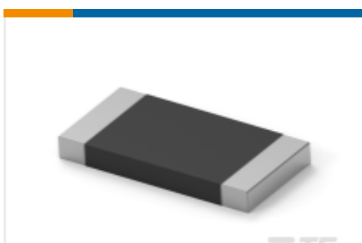
TE 产品编号7-2176422-6 TLRP 2512 3.0W R100 1% 50PPM 4K RL
