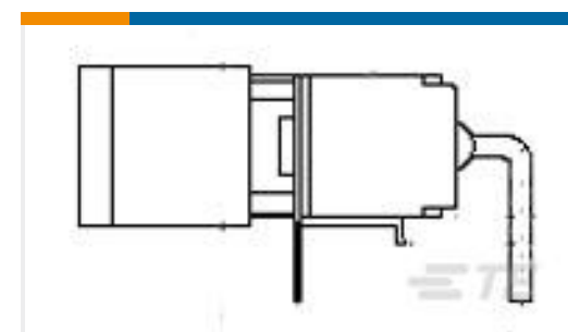
TE 产品编号1571986-8 A101J1AQ004=SGL POLE,ROCKER
