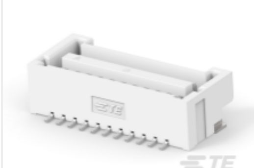
TE 产品编号2-2456589-2 Header Assy, 22pos, VT, KeyA, SGI 1.25
