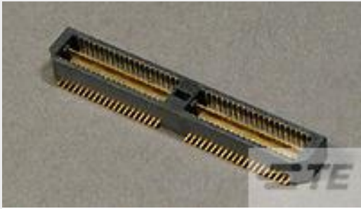
TE 产品编号 5-1658463-2 MSB0.80PL5ASY56DP,GP,30,VCTR
