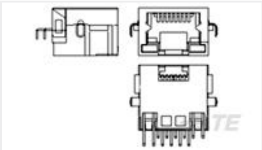
TE 产品编号2041411-1 RJ45 w/ LED, Tab Up, Offset, DIP, H=9.45
