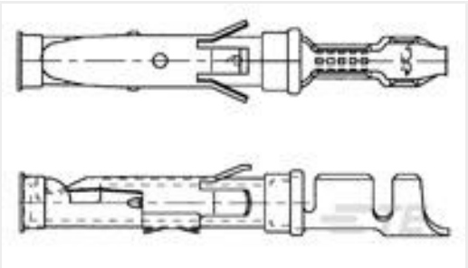
TE 产品编号163092-2 .062 DIA SOCKET ASSY 3+ (LP)
