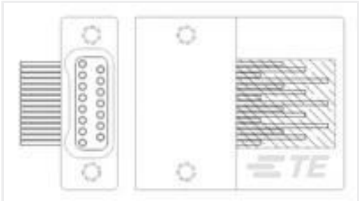
TE 产品编号1589487-9 STL025M6 = THRU-HOLE
