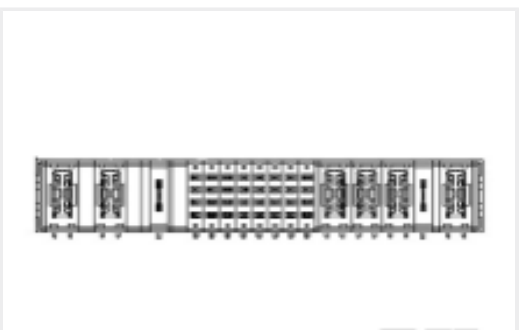
TE 产品编号2314578-1 R/A HEADER, MULTI-BEAM XLE, VITA 62
