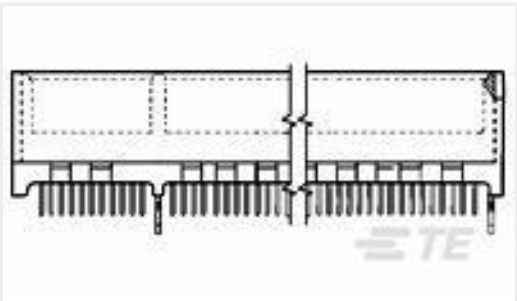
TE 产品编号5145167-4 STANDARD EDGE .050 SERIES 60 DUAL ASSY
