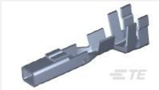
TE 产品编号177914-1 AMP POWER DBL LOCK REC (S)
