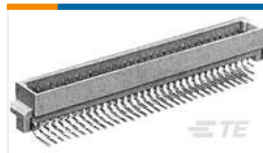
TE 产品编号5650473-5 ASSY,PIN,EUROCARD,TYPE C,LEAD-RL
