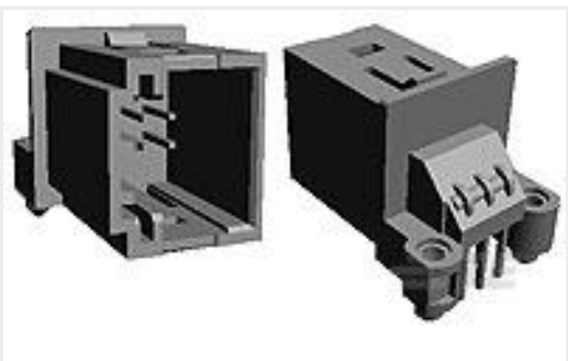
TE 产品编号953440-1 6pos MQS .63 header 90deg
