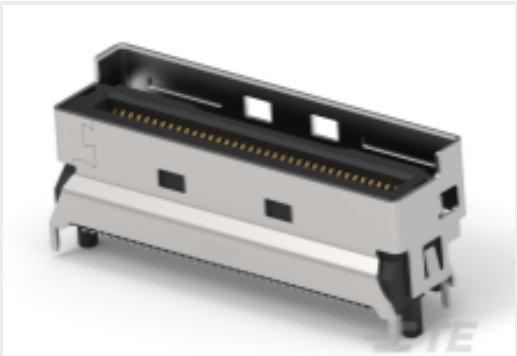
TE 产品编号1-2379397-7 MCIO INTERGRATED CONN, V/T,8X, SMT TYPE
