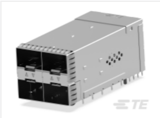
TE 产品编号2343522-7 SFP56 STACKED 2X2 RECEPTACLE ASSEMBLY
